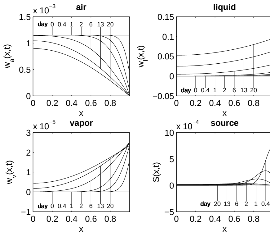
Figure. Graphs of the air, liquid and saturated vapor concentrations w_a , w_l , w_v , and the source S .
